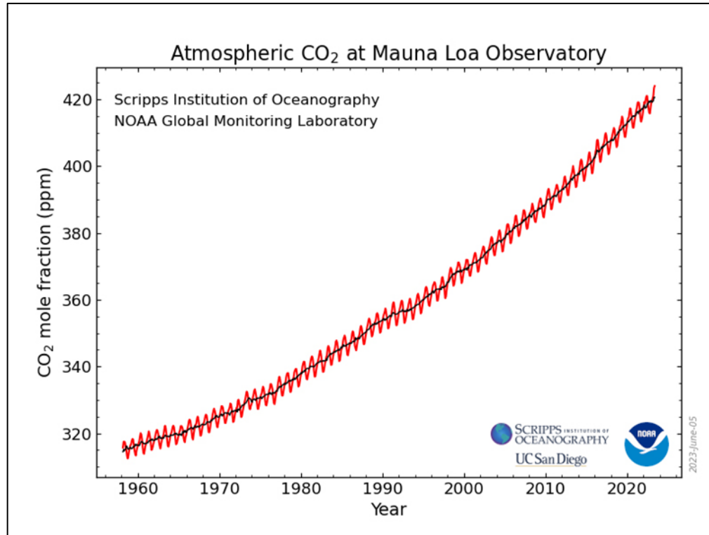
Graph from the National Oceanic and Atmospheric Administration (NOAA)
